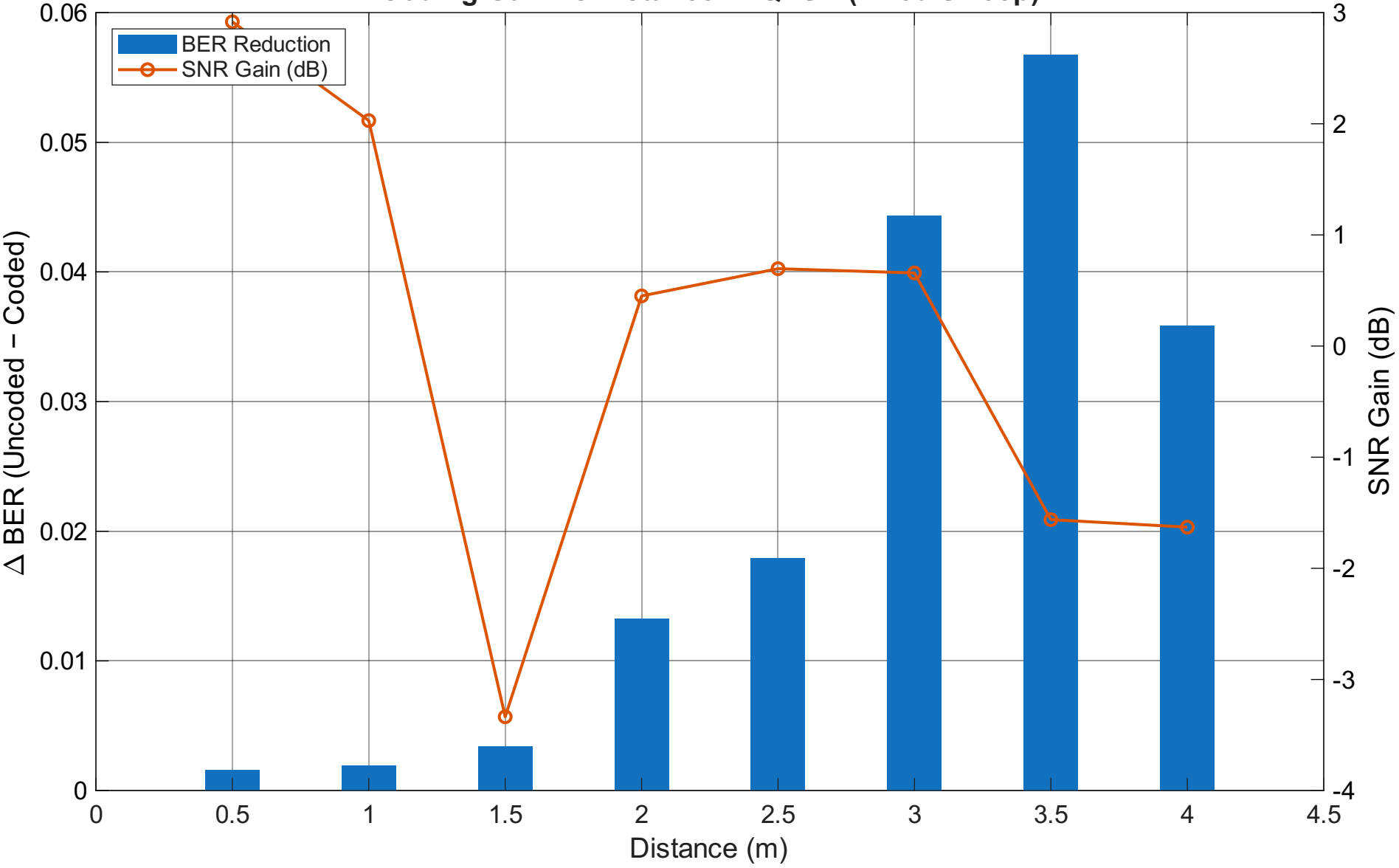
Coding Gain vs Distance — QPSK (Fixed Sweep)
