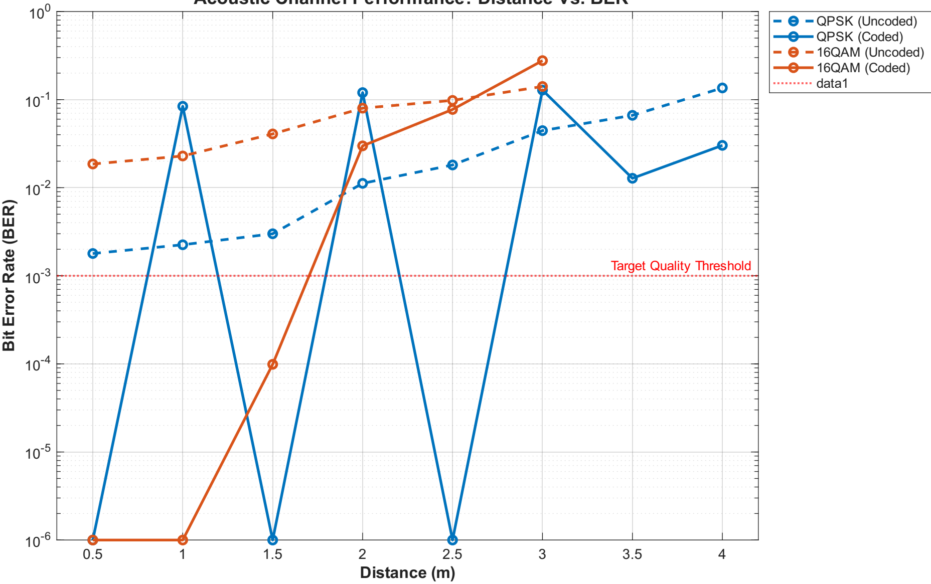
Acoustic Channel Performance: Distance vs. BER
