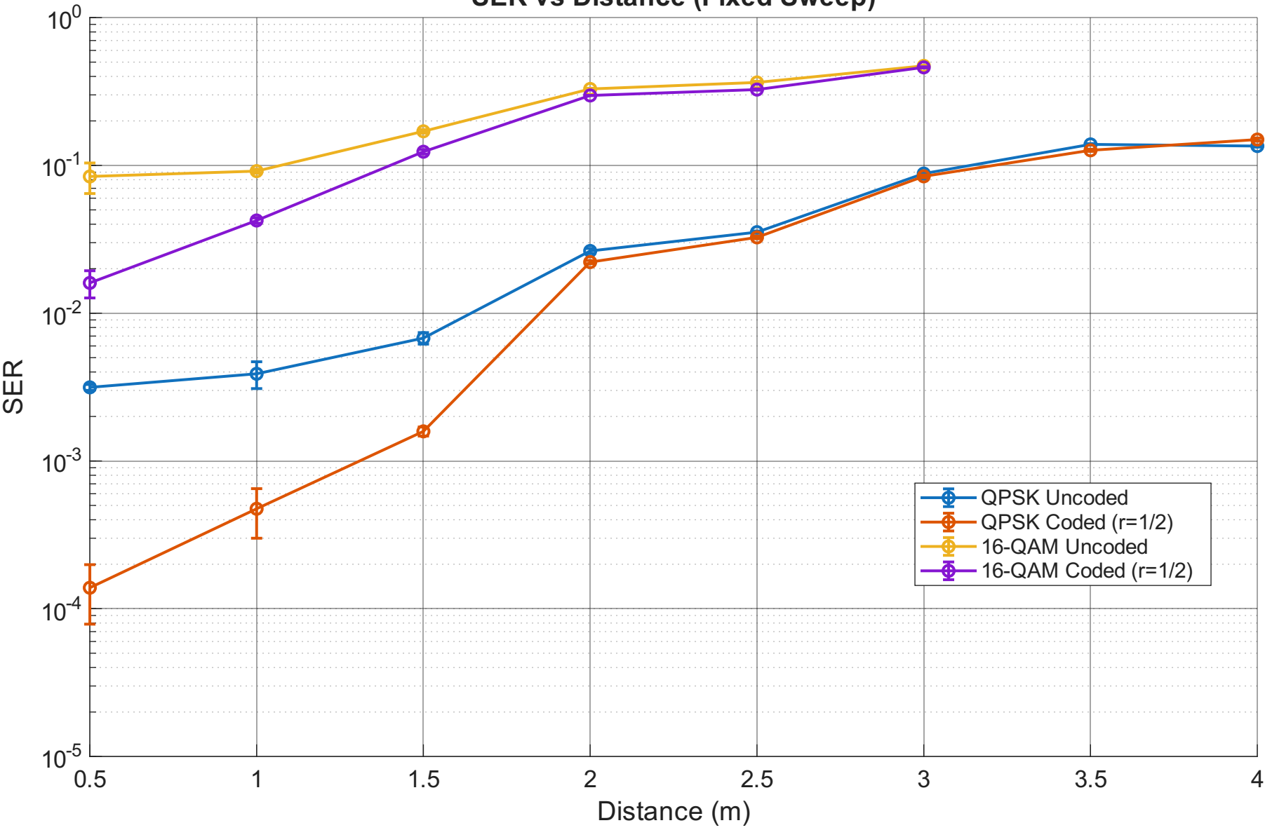
SER vs Distance (Fixed Sweep)
