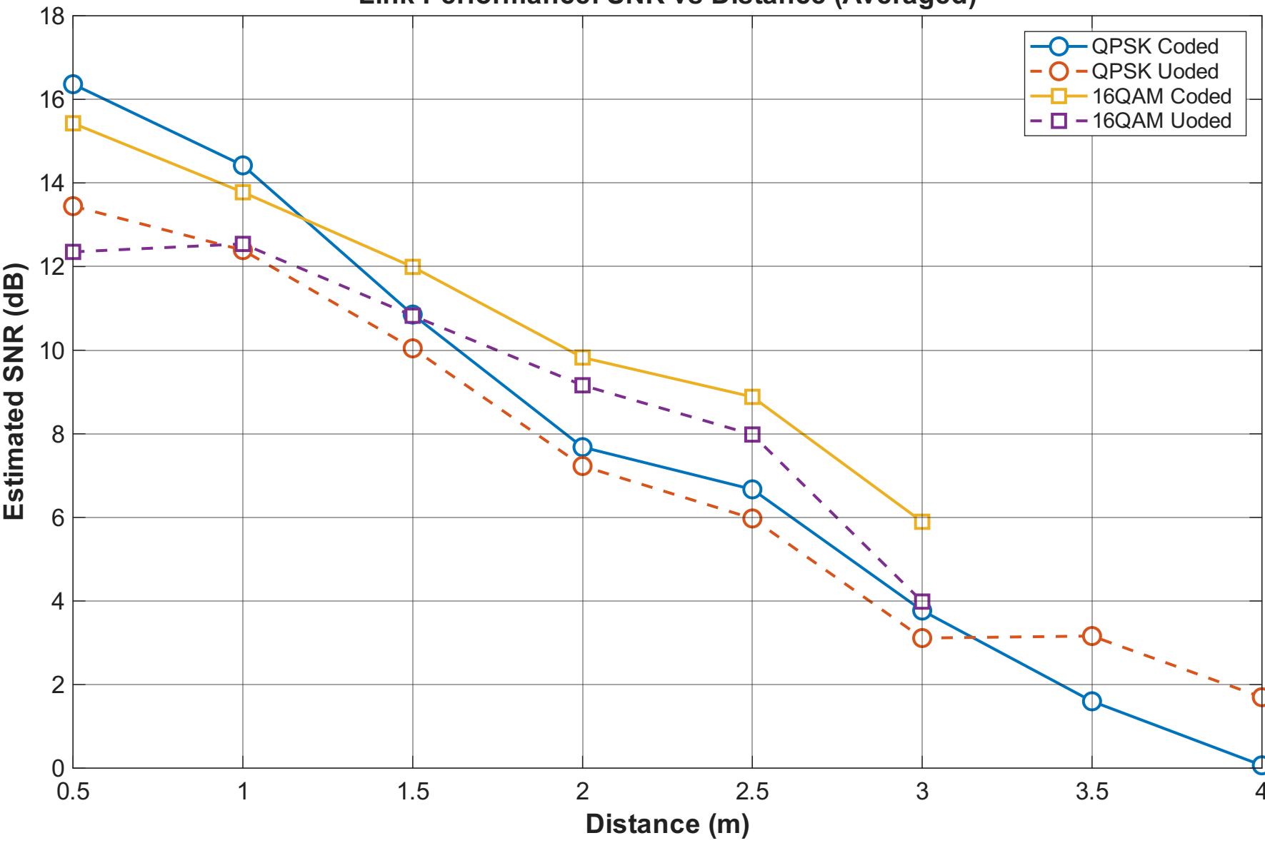
Link Performance: SNR vs Distance (Averaged)
