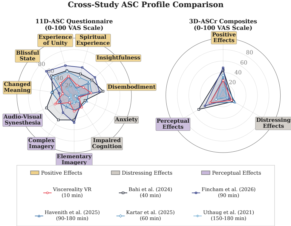
Fig. 9 Descriptive cross-study comparison of the present dataset with five named breathwork datasets. The left panel shows 11D-ASC subscale means and the right panel shows 3D-ASCr composite means. The Viscerality profile pools the symmetric and asymmetric VR conditions. Lines show raw 0–100 profile means, not standardized effect sizes; differences in technique, duration, sample, music, facilitation, and study design preclude inferential comparison. Legend order is purely graphical and does not imply a numbered study sequence.
