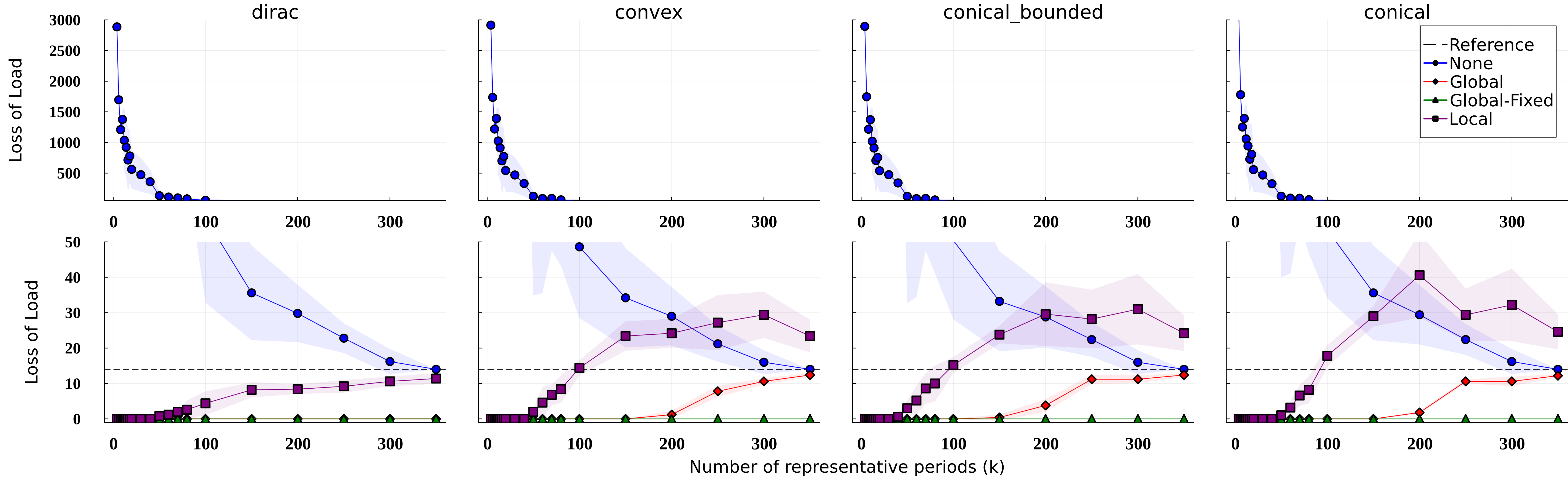
Loss of Load vs number of RPs (k) using k-means
