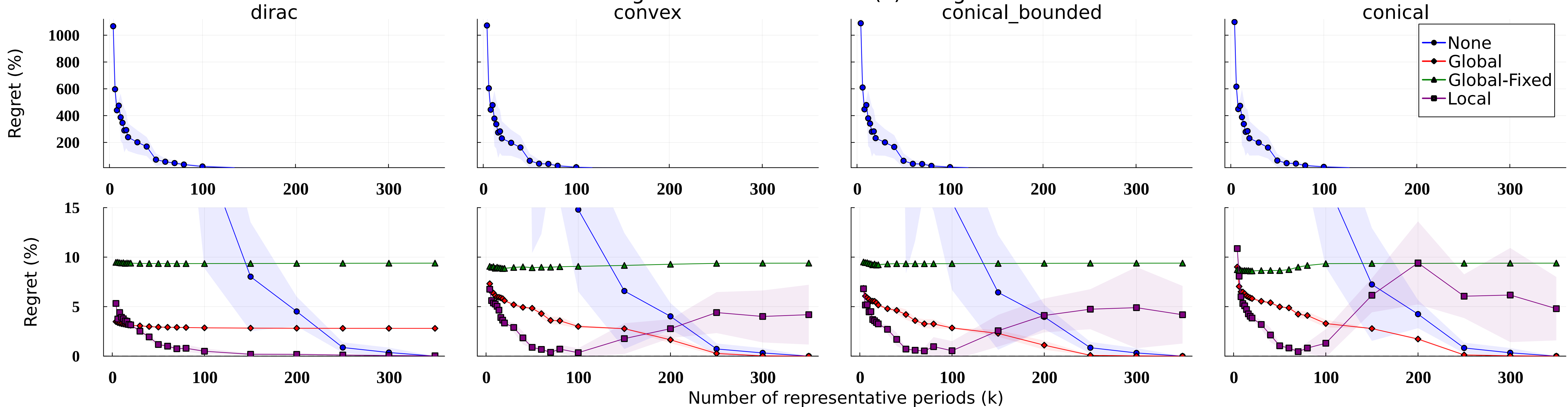
Regret vs number of RPs (k) using k-means
