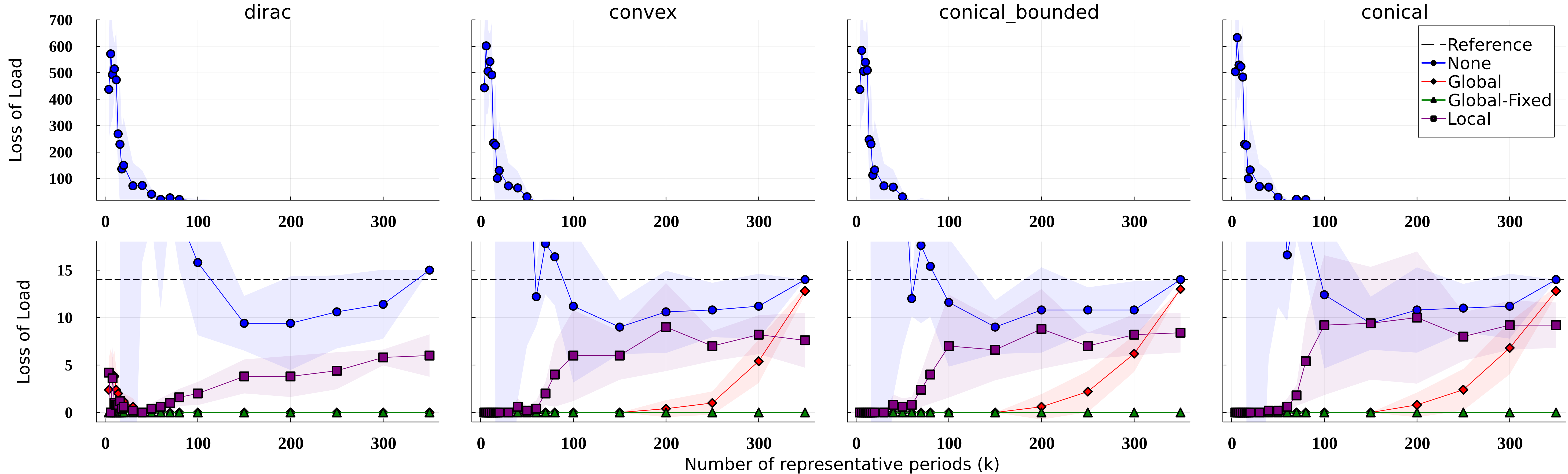
Loss of Load vs number of RPs (k) using k-medoids
