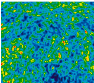
A patch of the real microwave sky. Hot and cold spots differ by about 0.0001 °C. NASA / WMAP, public domain.
