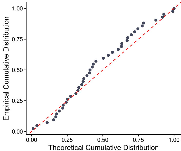
P-P Plot
