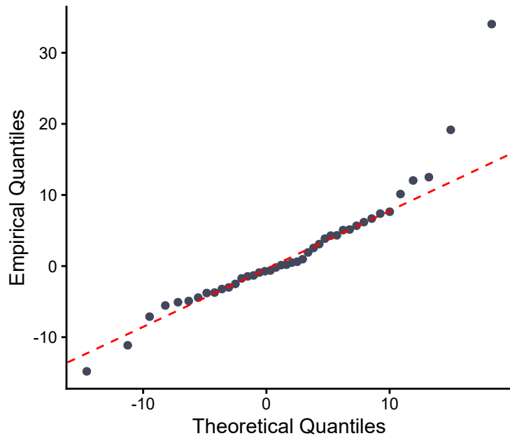
Q-Q Plot
