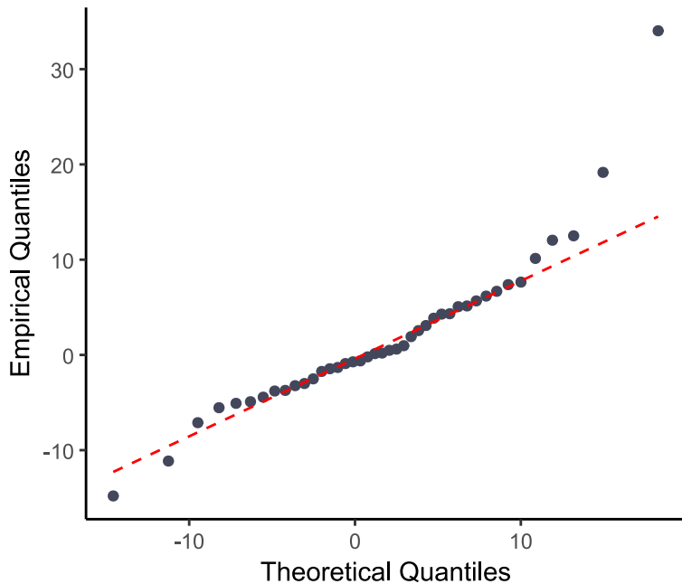
Q-Q Plot
