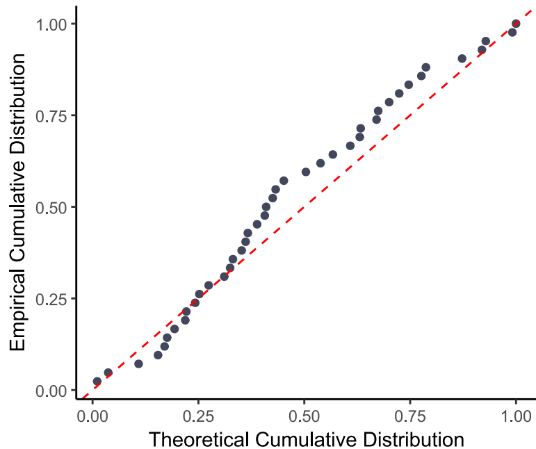
P-P Plot
