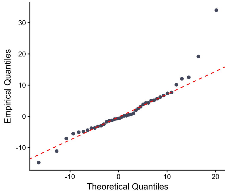
Q-Q Plot
