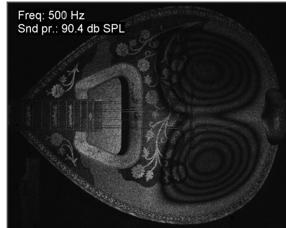
(c) 1_2 500 Hz
