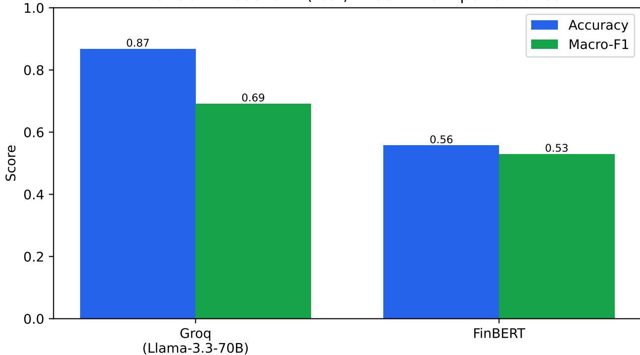
Financial PhraseBank (test) — sentiment performance
