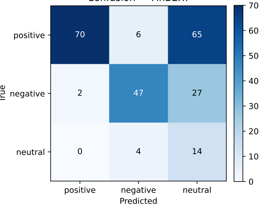
Confusion — FinBERT
