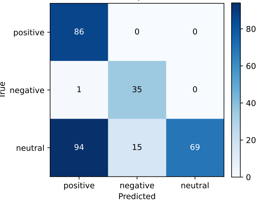
Confusion — Groq (Llama-3.3-70B)
