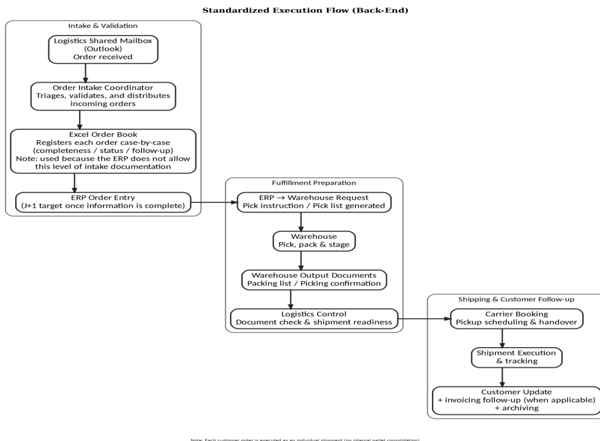
Figure 2 – Standardized execution flow (back-end)
