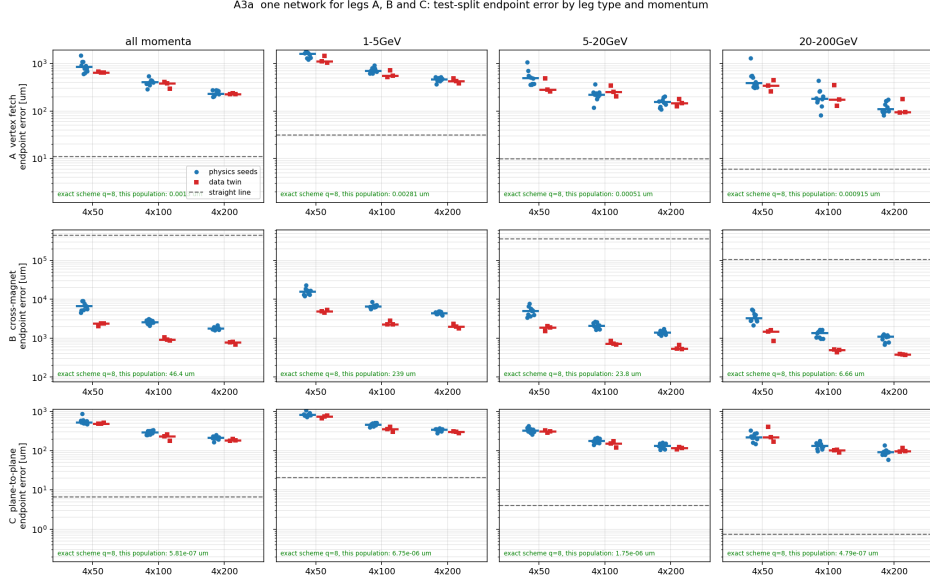
Figure 7: Test-split endpoint error for the single general network with absolute outputs, by leg type (rows: A vertex fetch, B cross-magnet, C plane-to-plane) and momentum band (columns: all momenta, then 1 to 5, 5 to 20 and 20 to 200 GeV), on a logarithmic vertical axis. Blue circles are the ten label-free seeds and red squares the three supervised seeds, with horizontal bars at the median; the dashed grey line in each panel is the straight-line baseline and the green annotation gives the exact-scheme ceiling on that same population. The middle row shows the network beating the straight line by two orders of magnitude on the cross-magnet leg while sitting a factor 56 above the ceiling; the top and bottom rows show the opposite situation, where the straight line lies below every network point.
