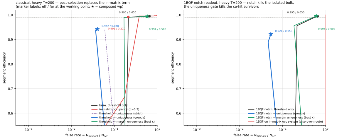
Figure 6: The hit-uniqueness gate: composed threshold→gate frontiers against the base and in-matrix-occupancy sweeps, classical (left) and 1BQF (right), heavy T = 200 . The gate reaches false-rate levels the in-matrix term cannot, at either solver.
