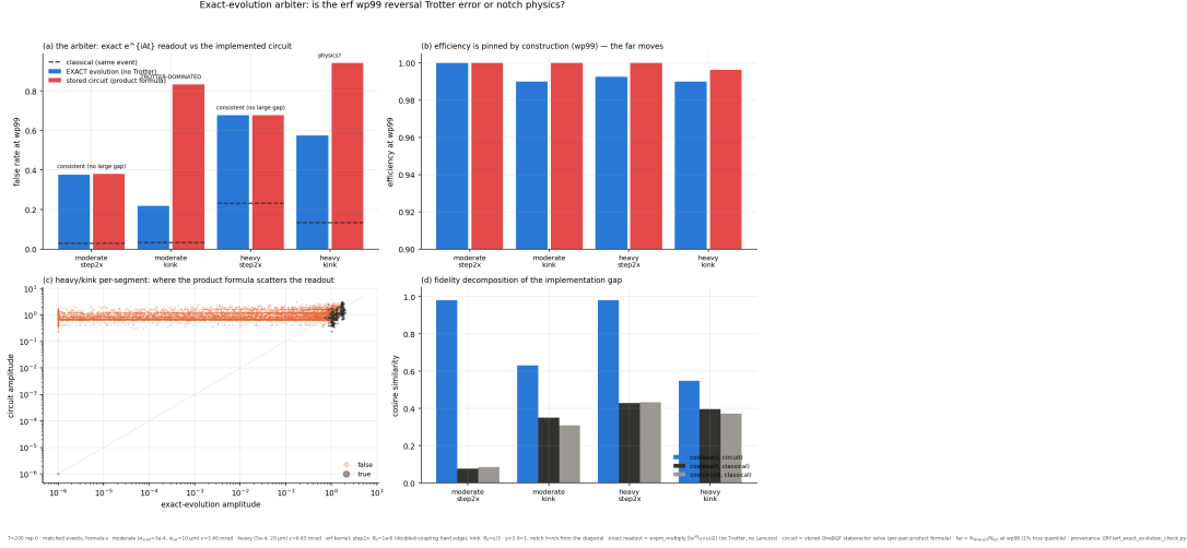
Figure 9: The exact-evolution arbiter on the erf angular-cost Hamiltonian: uniform-coupling kernels (step2x) show circuit = exact (the deficit is physics); finite-width kernels (kink) are Trotter-dominated — removing the product formula collapses the false rate from 0.83 to 0.22 (moderate) and 0.94 to 0.58 (heavy).
