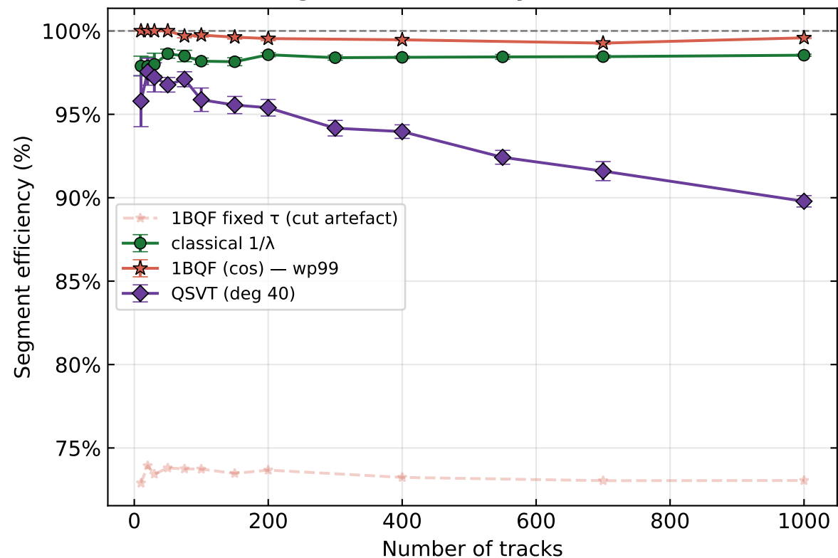
i) Segment efficiency N_{\text{true act}}/N_{\text{true all}}
