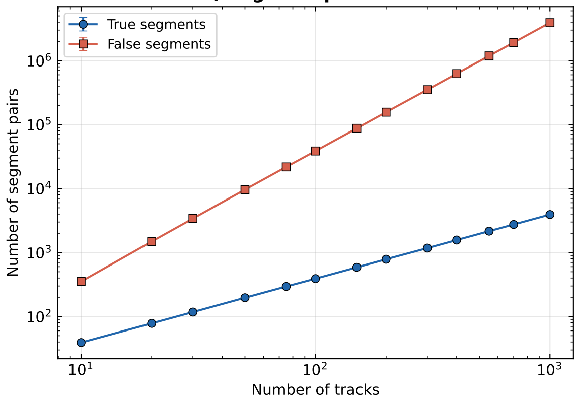
iii) Segment-pair counts
