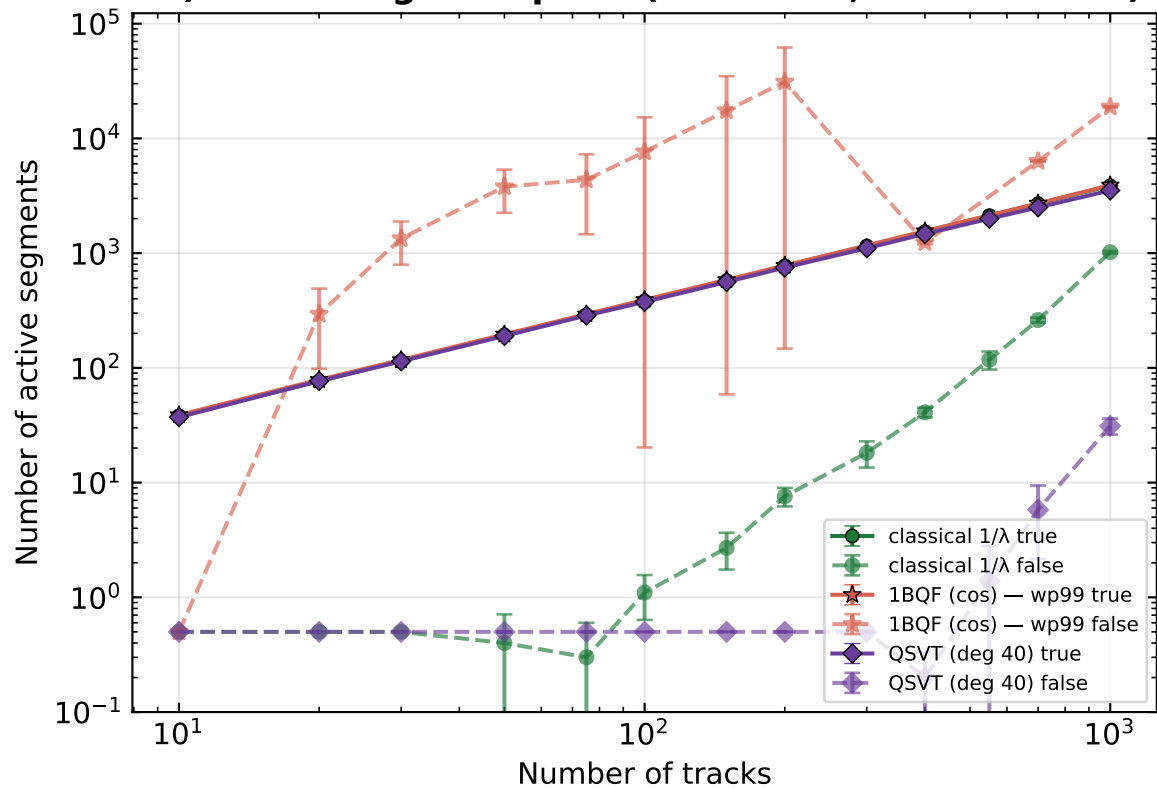
iv) Active segment pairs (solid true, dashed false)
