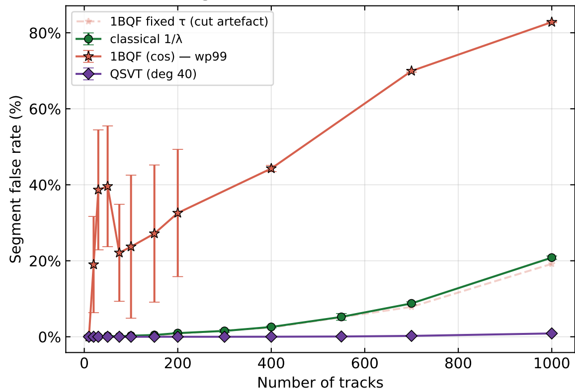
ii) Segment false rate N_{\text{false act}}/N_{\text{active}}
