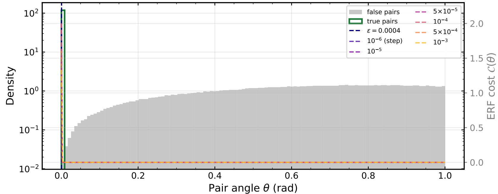
Pair angle distributions with ERF cost — \sigma_s = 0.0001
