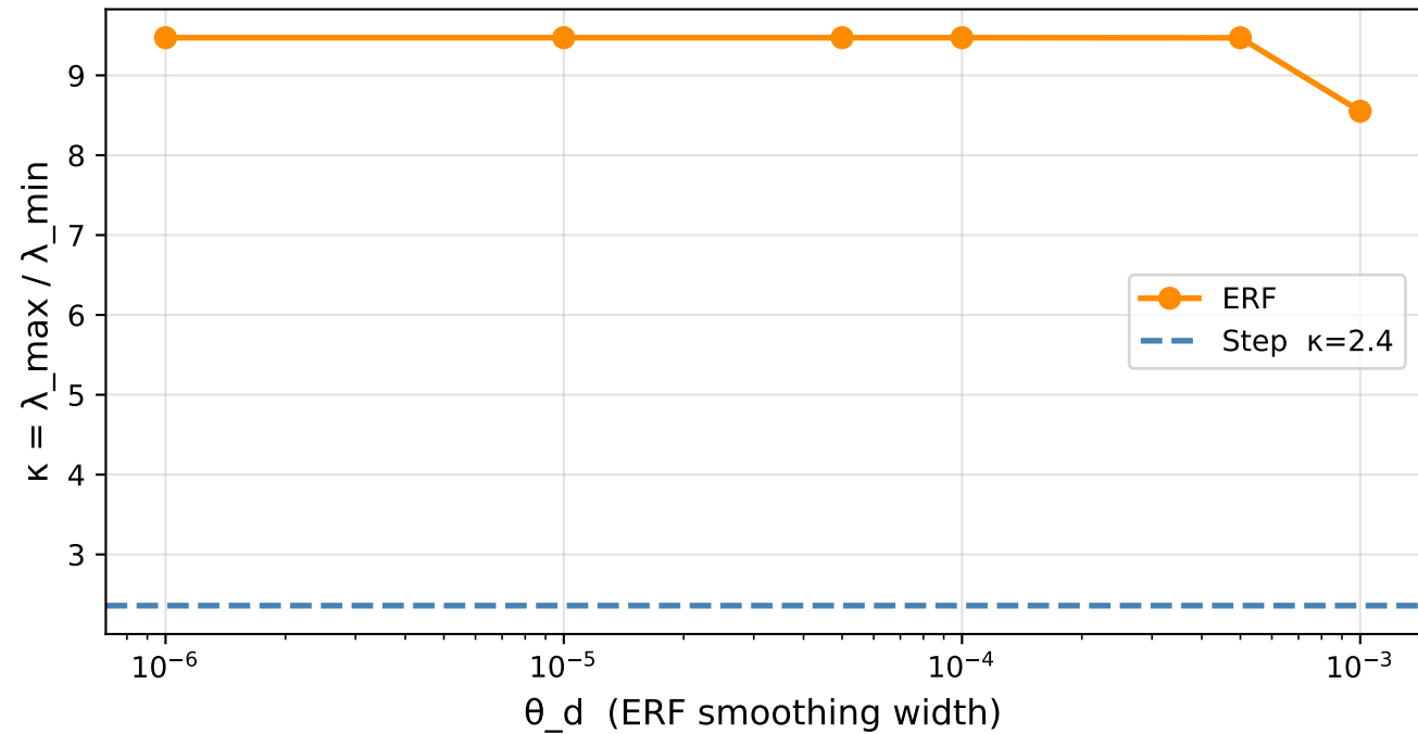
Condition number vs ERF smoothing (T=20, clean)
