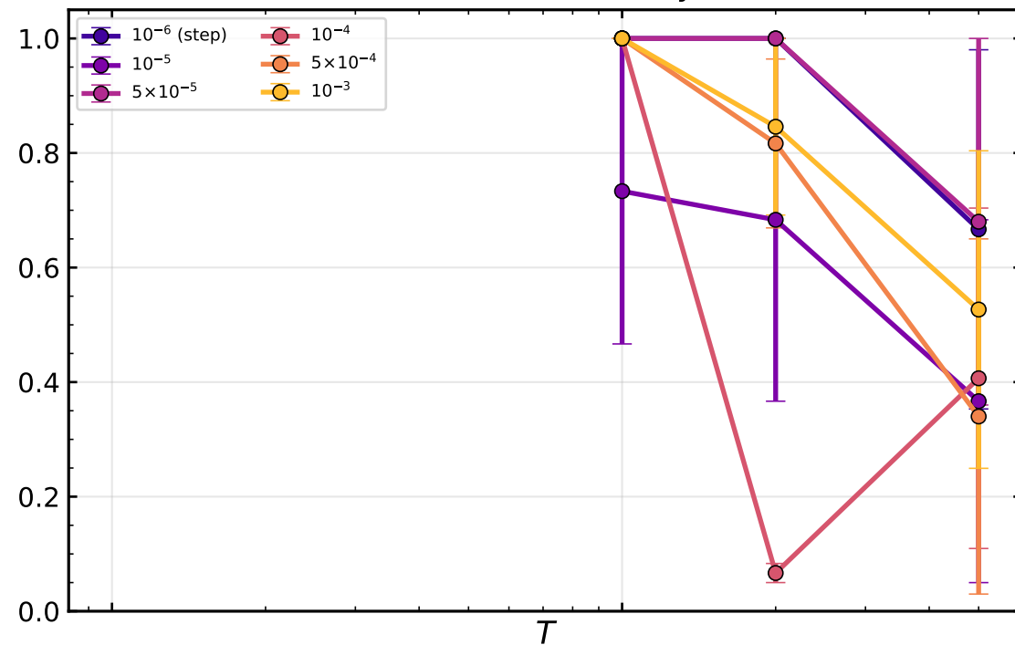
Classical efficiency
