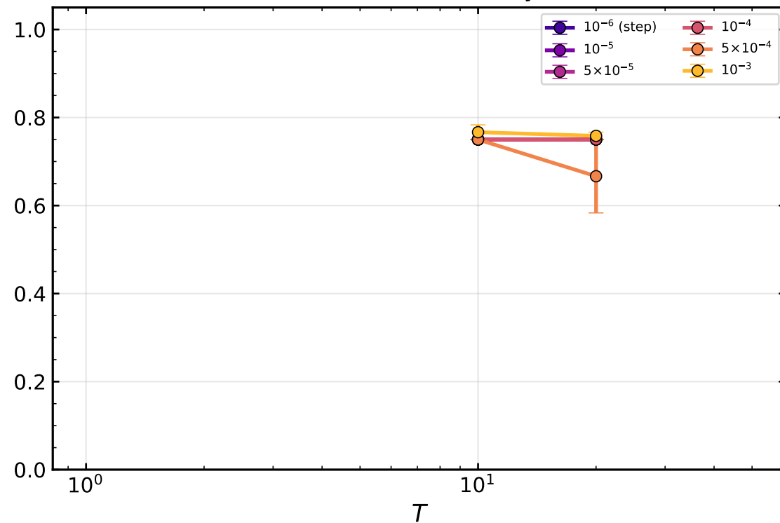
Quantum efficiency
