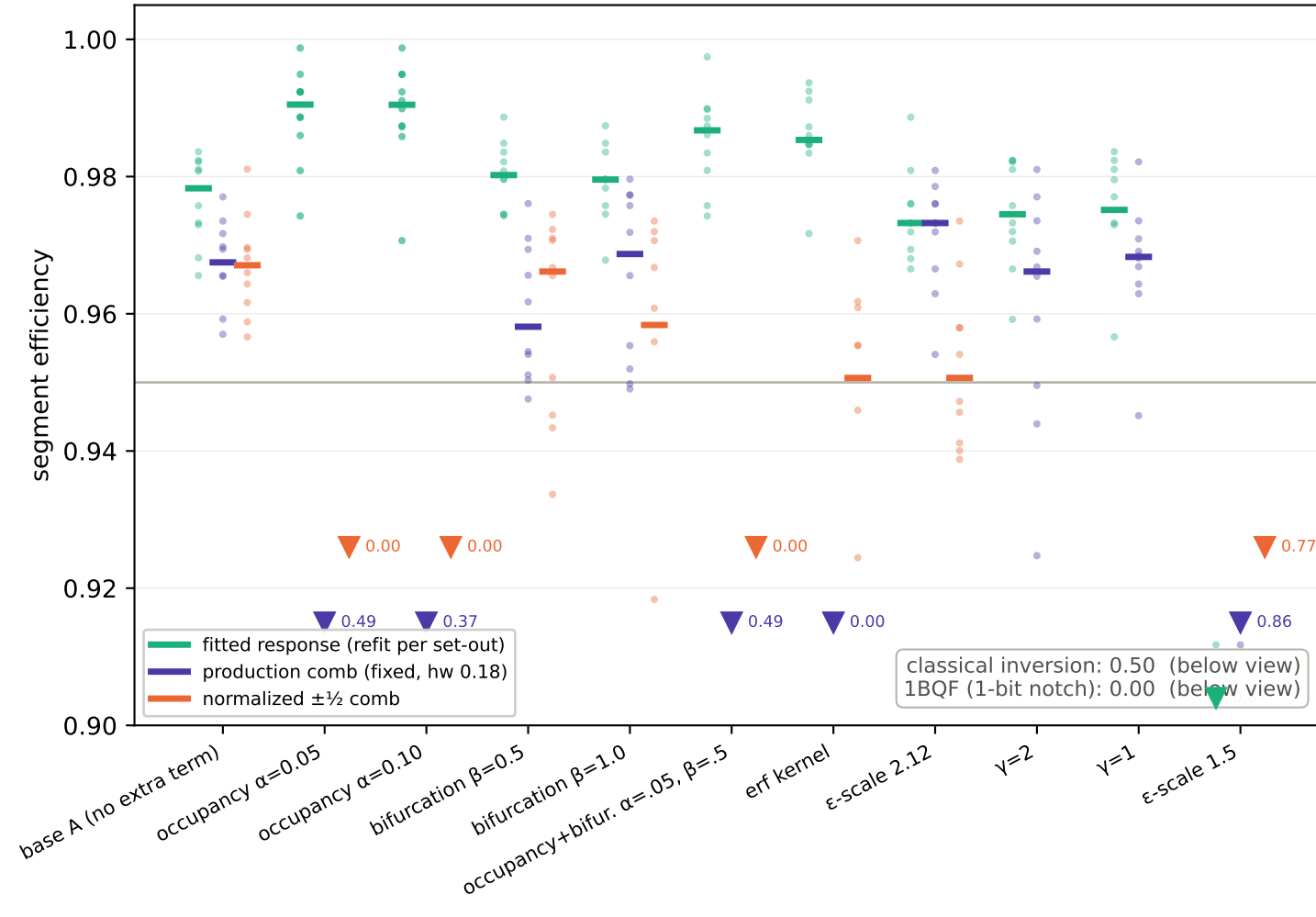
(a) efficiency you can buy at far \leq 1\% ( \blacktriangledown = collapsed below view)
