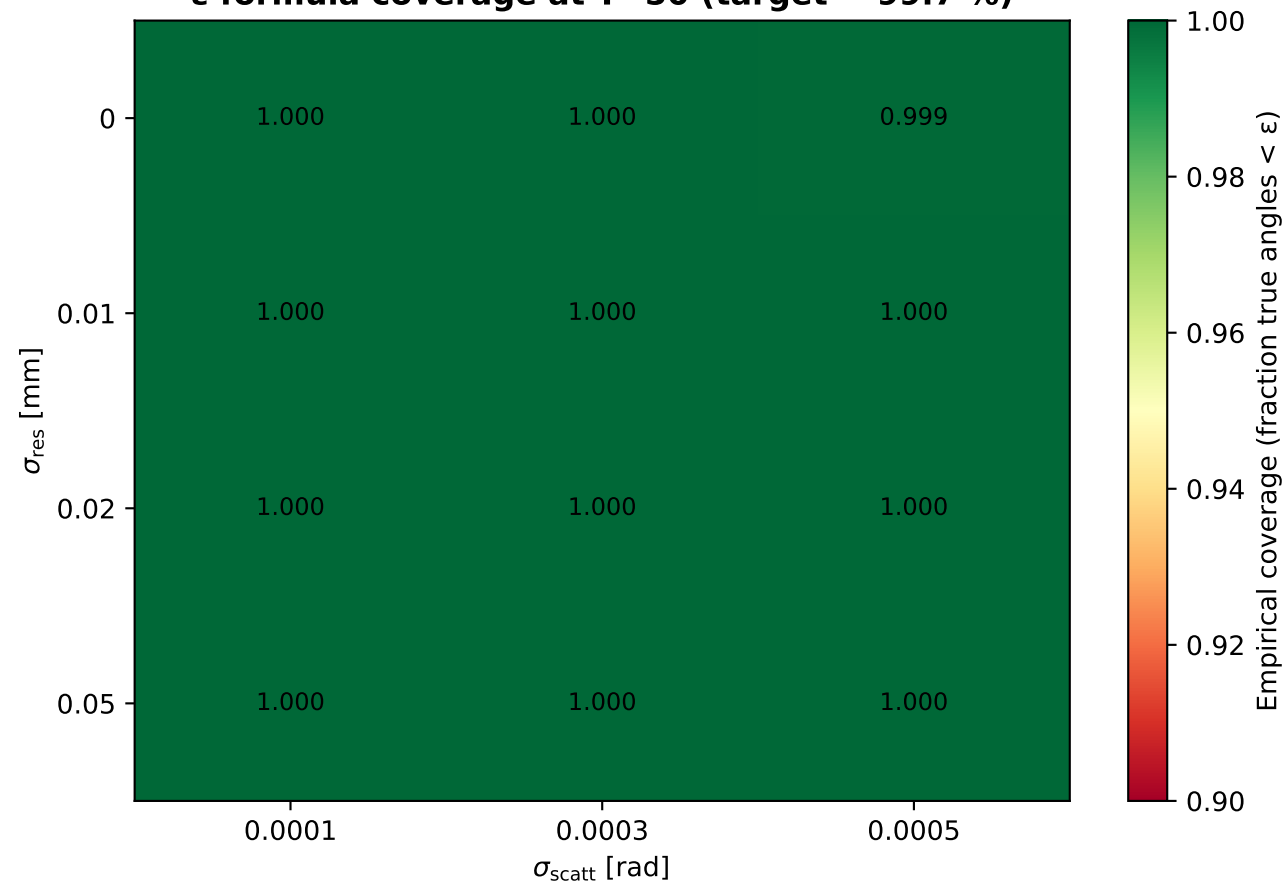
\varepsilon formula coverage at T=50 (target = 99.7 %)
