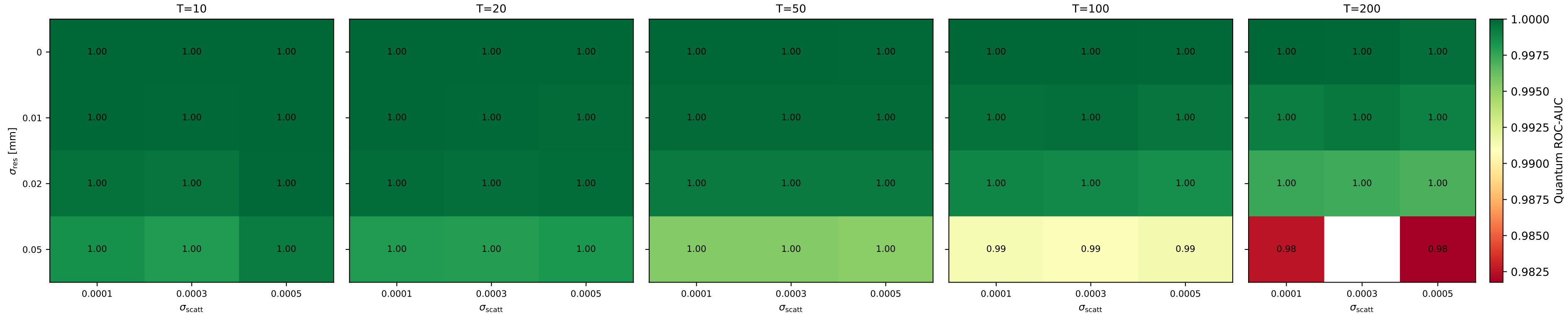
Quantum ROC-AUC over noise grid
