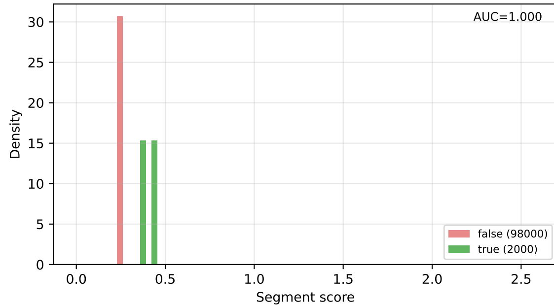
Classical solver
