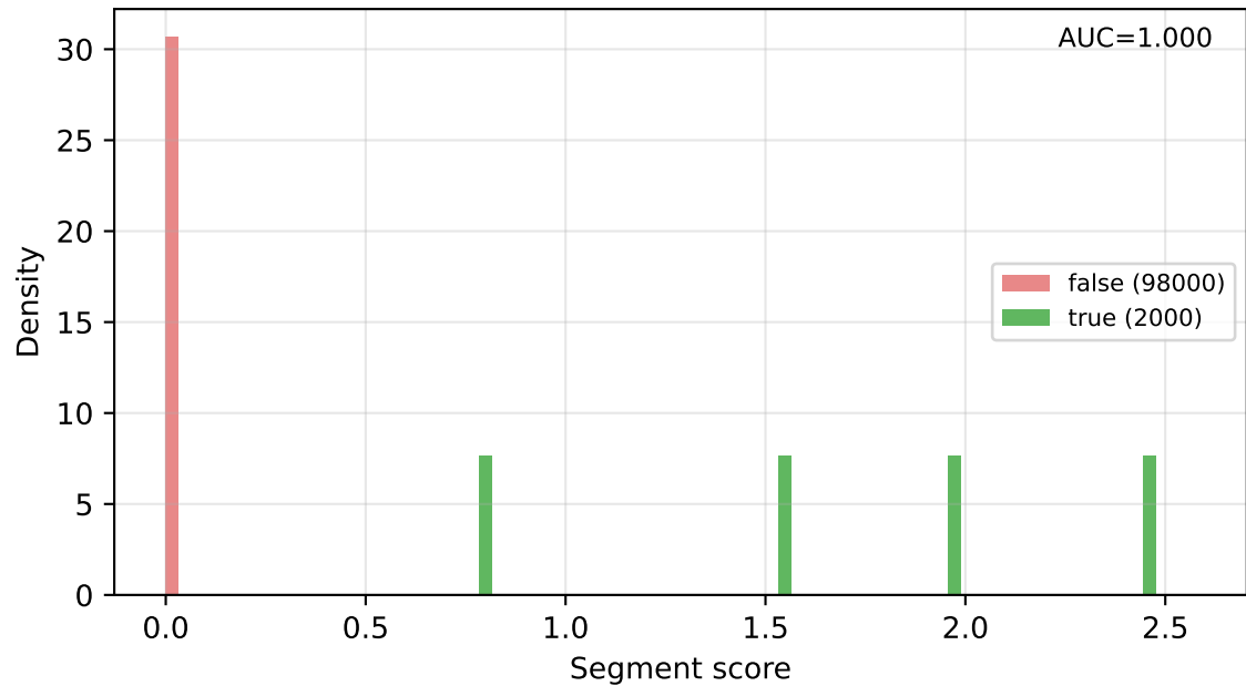
Quantum solver
