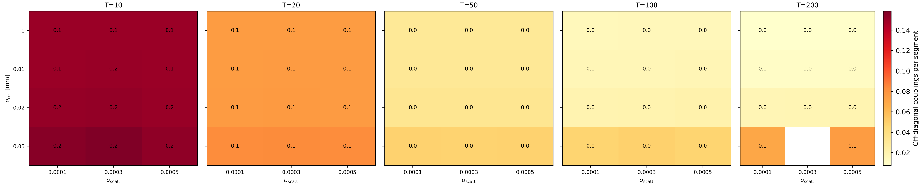
Matrix A density: off-diagonal fill vs noise
