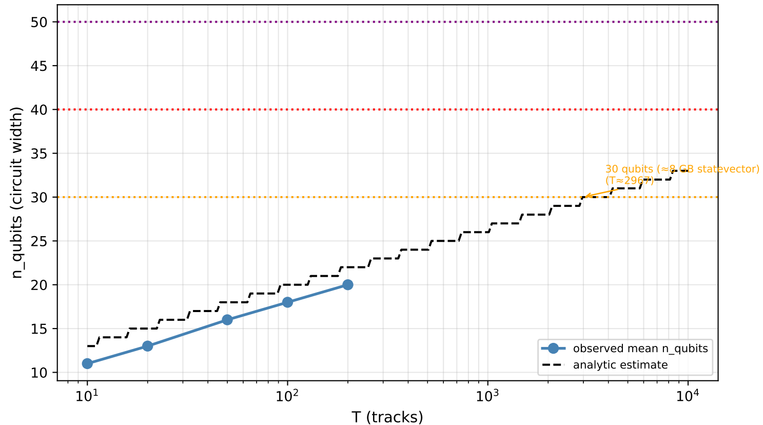
Quantum circuit width vs T (statevector memory scales as 2^{n_{\text{qubits}}} complex128)
