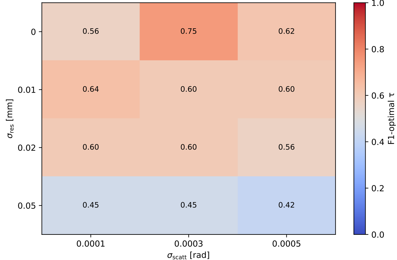
Classical: F1-optimal \tau at T=50 (default \tau=0.35 shown for reference)
