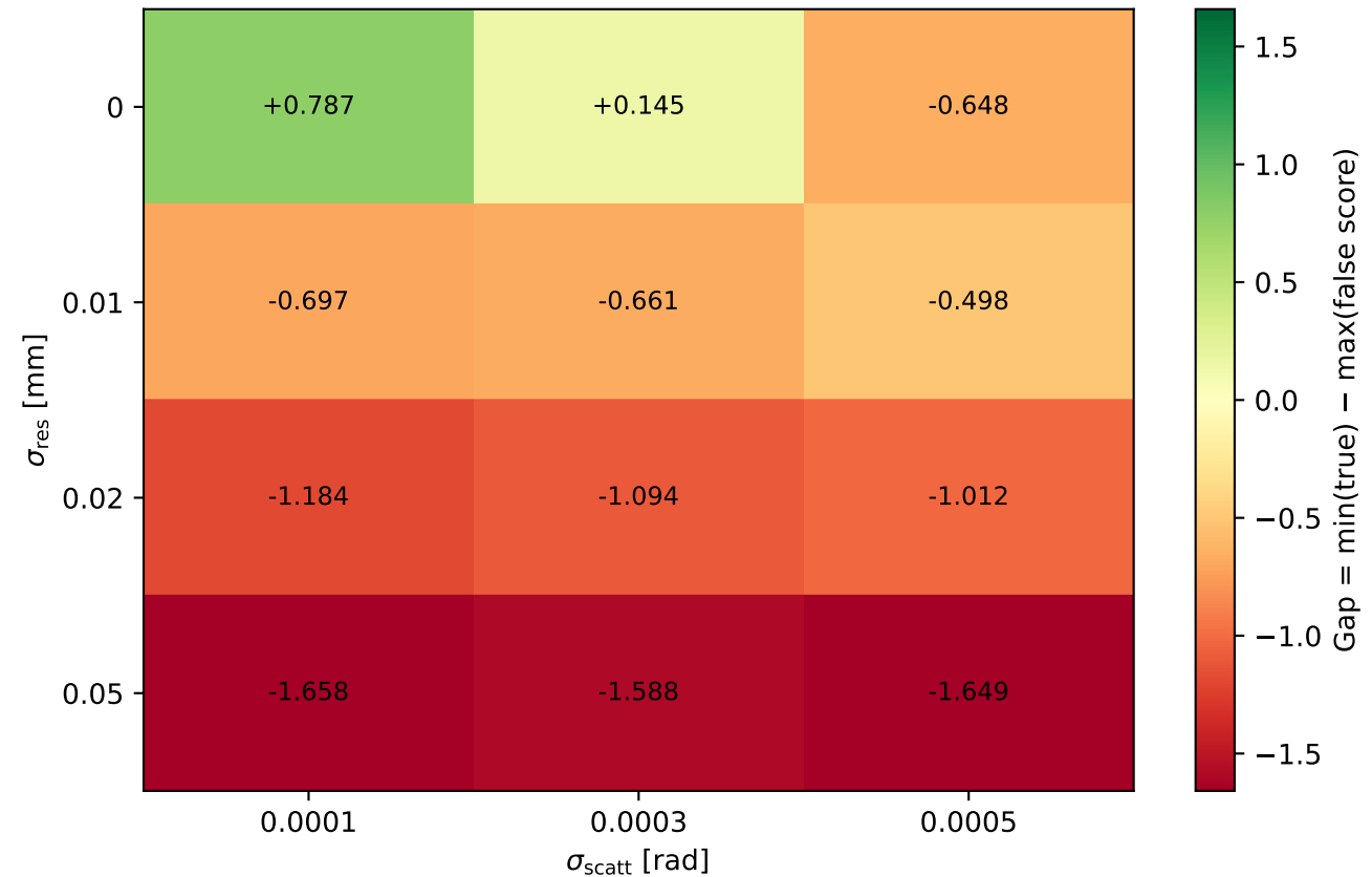
Quantum: true/false score separation gap at T=50 (green > 0 = perfect; red < 0 = false segments leak above zero)
