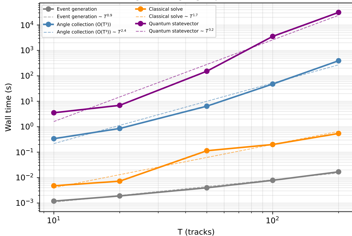
Timing vs T (log-log + power-law fits)
