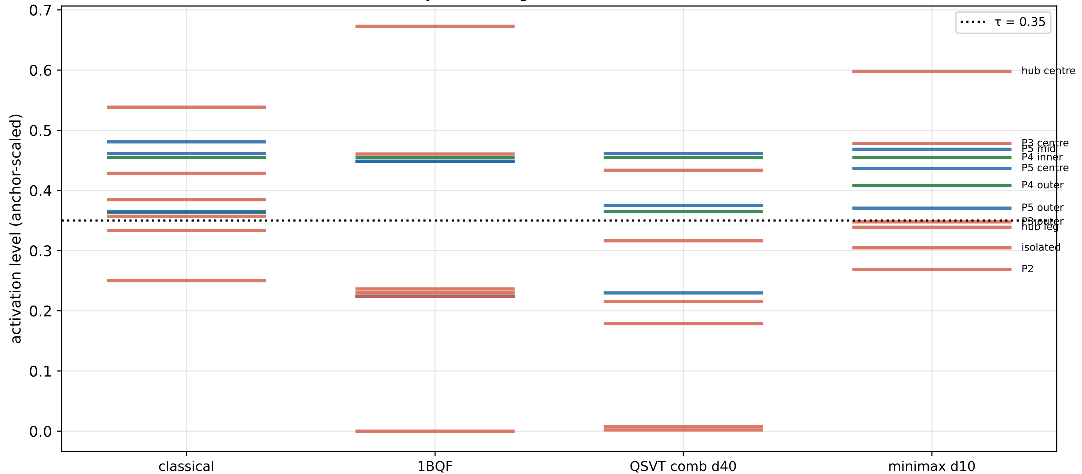
The activation ladder per filter — green true, red false, blue contaminated-P5
