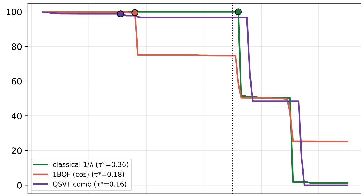
T = 400 (clean)
