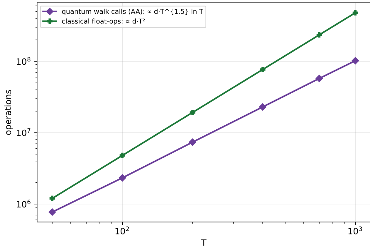
(b) WP6: the honest operation-count comparison
