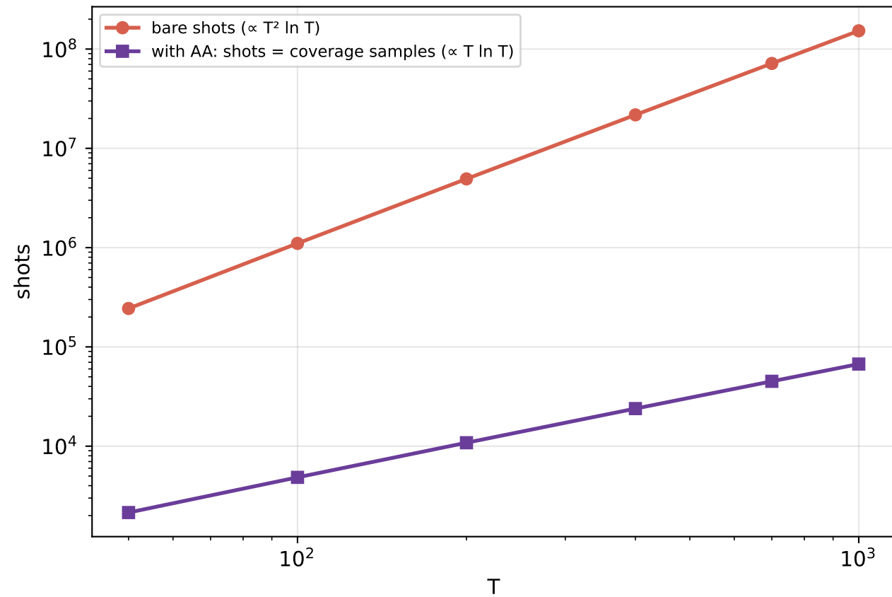
(a) WP3 shots budget for active-set readout
