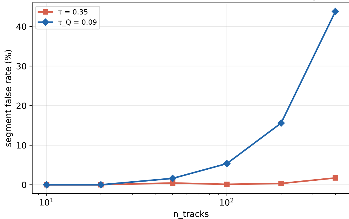
False rate: the cost is the 1BQF false tail at high n
