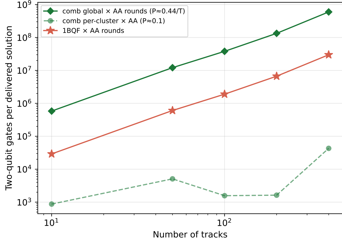
ii) With amplitude amplification
