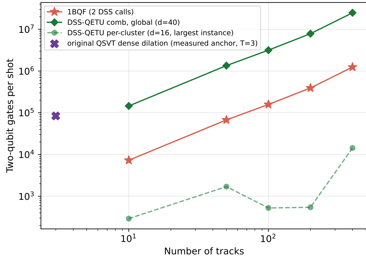
i) Per-shot 2q gates (structure-linear)
