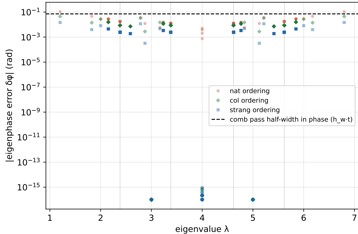
i) DSS product-formula phase error, T=400
