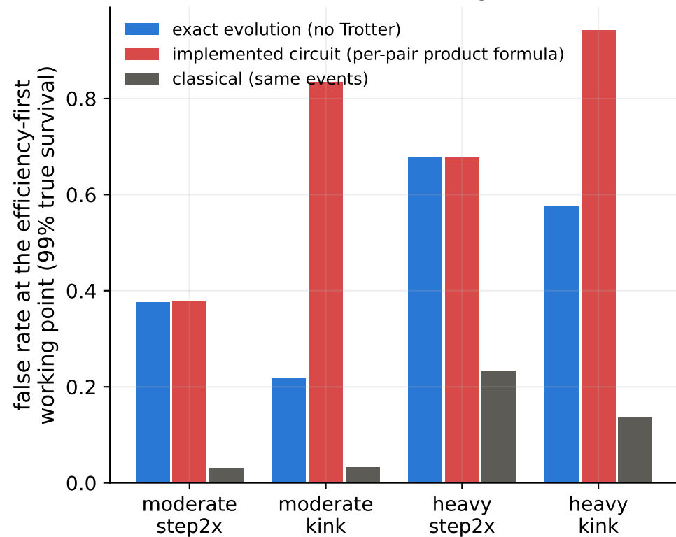
(a) circuit vs exact evolution, erf angular-cost Hamiltonian
