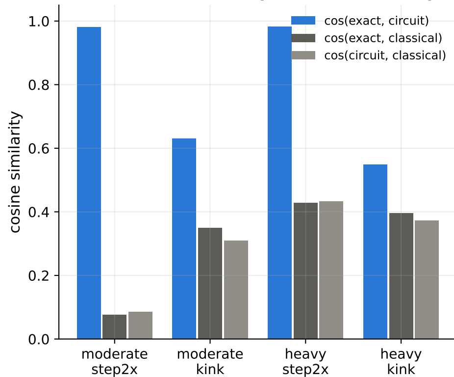
(b) where the readouts disagree: uniform kernels agree, weighted kernels are Trotter-dominated
