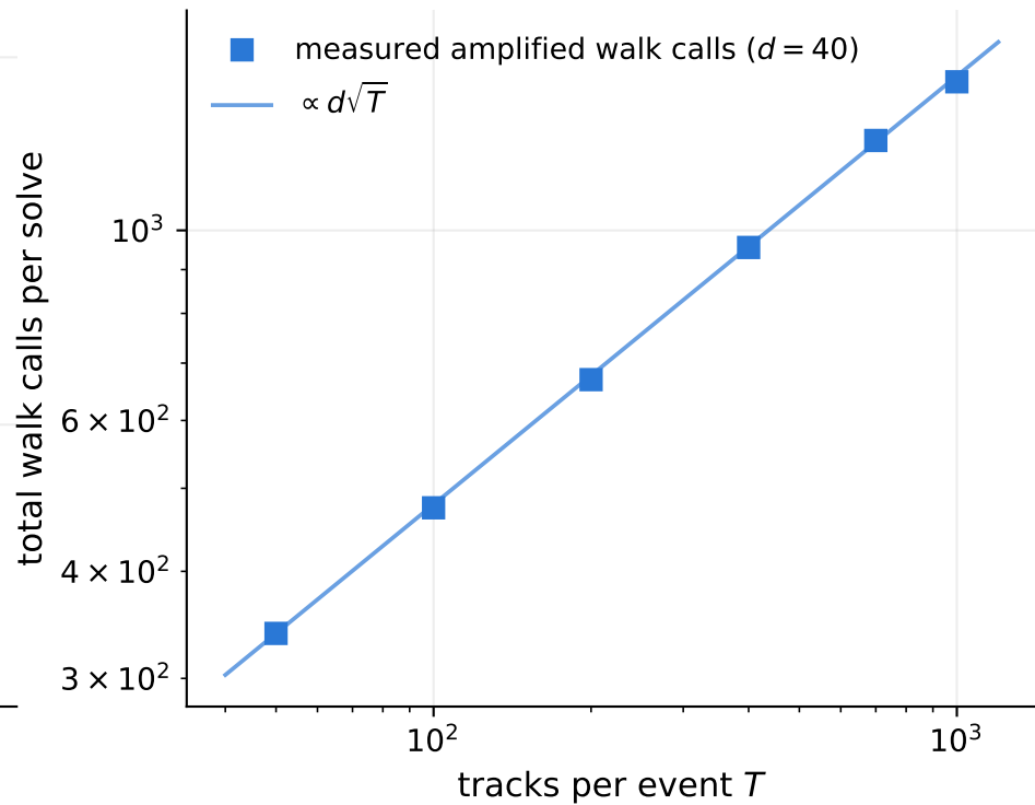
(b) walk-call budget after amplitude amplification
