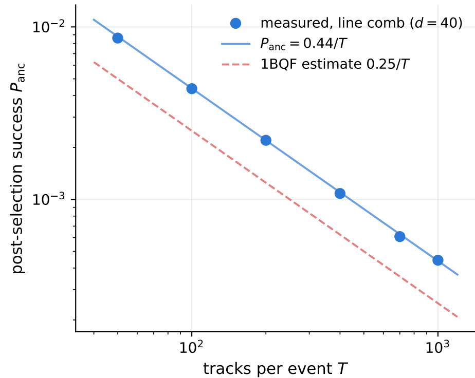
(a) success probability of one repetition
