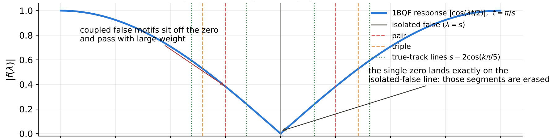
(a) the one-bit filter: one zero, spent on the largest false population
