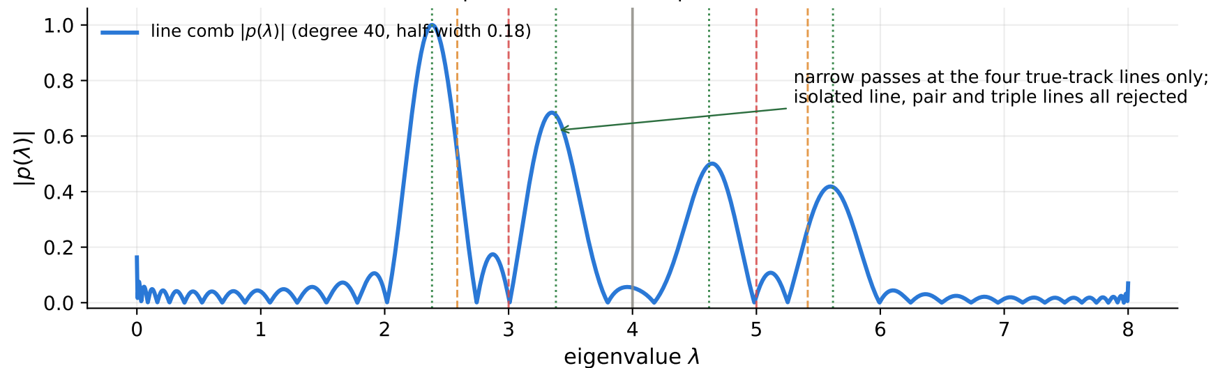
(b) the QSVT line comb: a zero (or a pass) wherever the spectrum needs one
