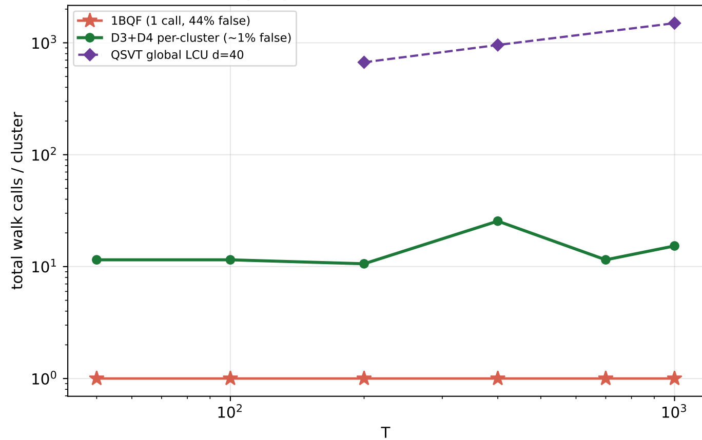
(b) depth: per-cluster \sim 10 calls, flat in T (no \sqrt{T} )
