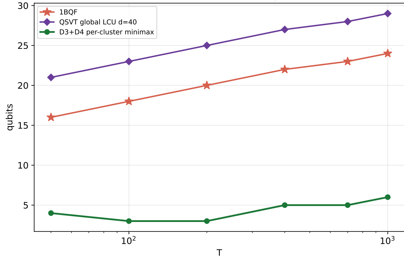
(a) qubits: D3+D4 \approx 5-6, below the global 1BQF
