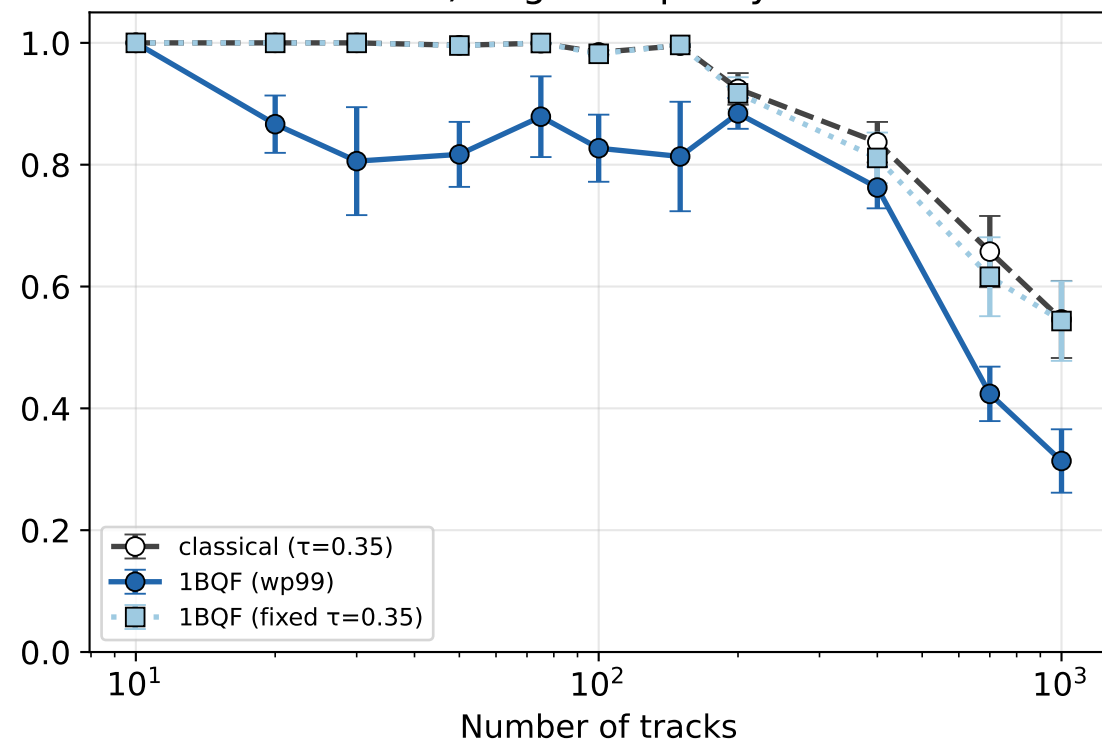
iv) Solver cosine fidelity
