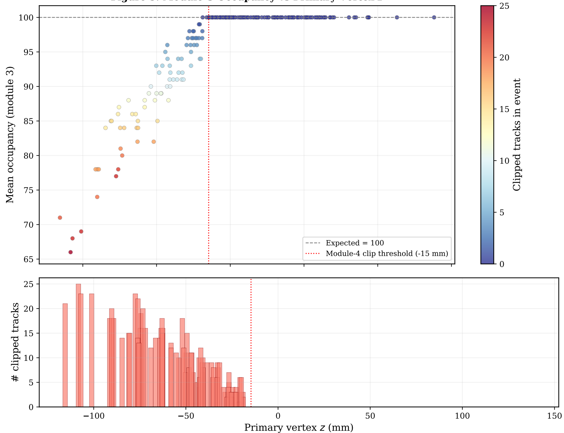
Figure 5: Module-3 Occupancy vs Primary Vertex z
