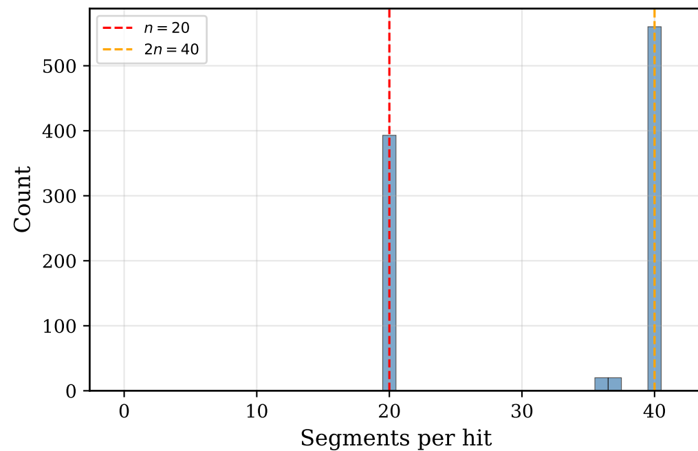
\pm 0.1 rad, 20 tracks (clean)
