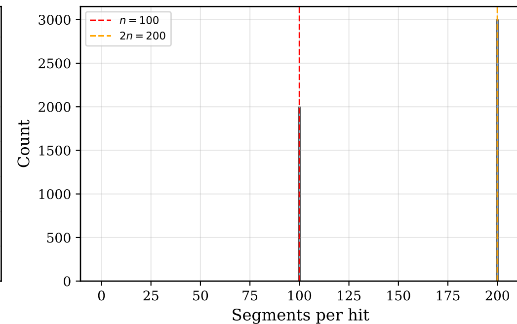
\pm 0.1 rad, 100 tracks (clean)
