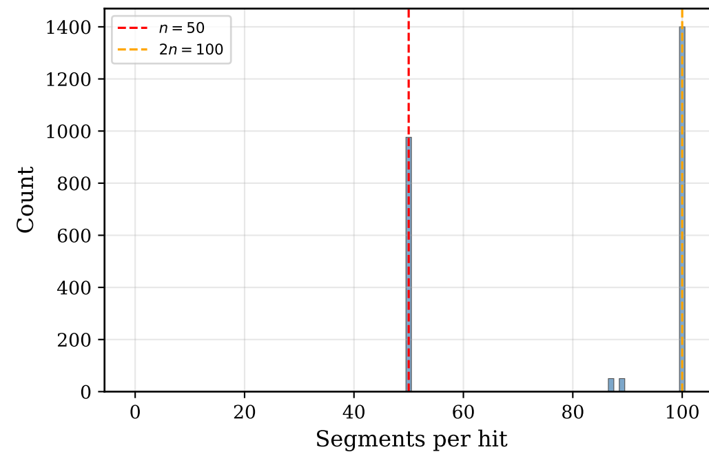
\pm 0.1 rad, 50 tracks (clean)
