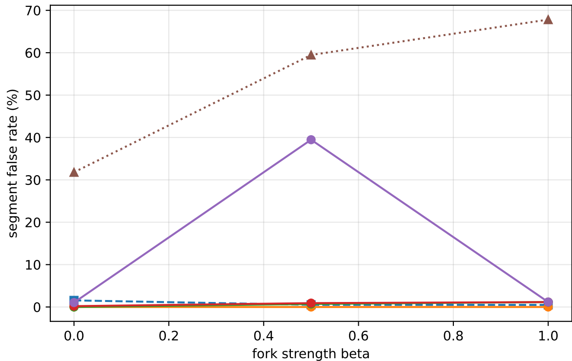
Composition on A'(beta): the comb at its own cut + occupancy gate (mean over T x reps)
