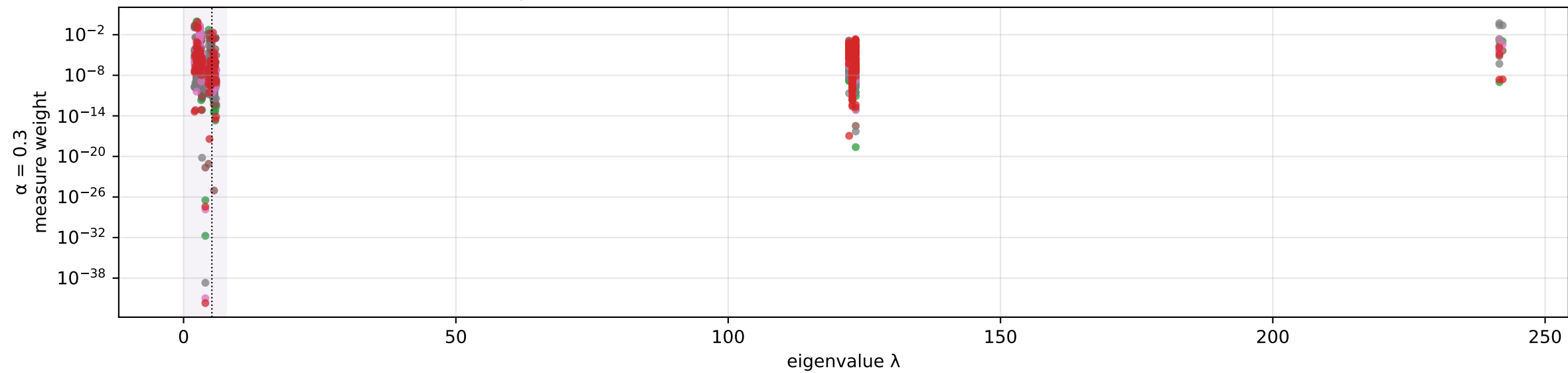
A'( \alpha=0.3 ): family spectral measures (shaded = current comb window s \pm 3.8 ; dotted = attractor s' = 5.2 )
