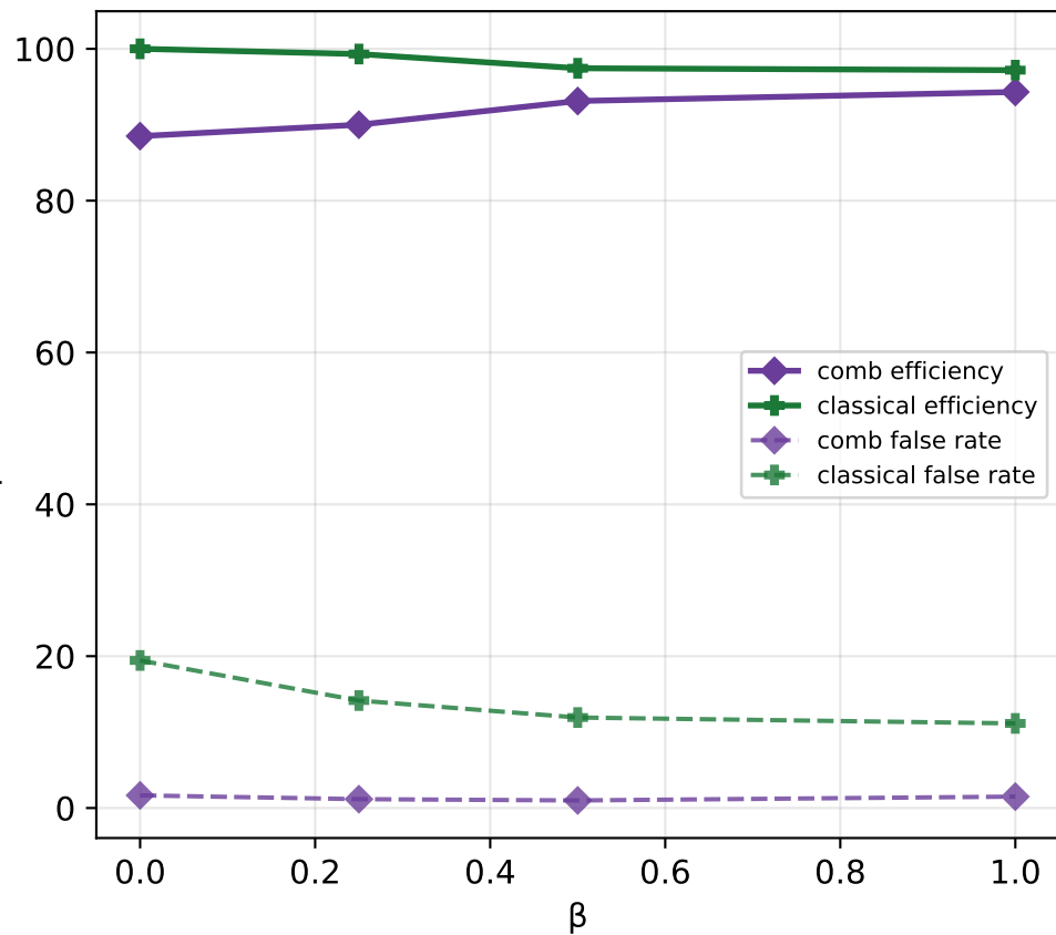
(a) \epsilon=4 mrad, T=400 (386 false actives at \beta=0 ): \beta recovers contamination + cleans classical; isolated bridges persist
