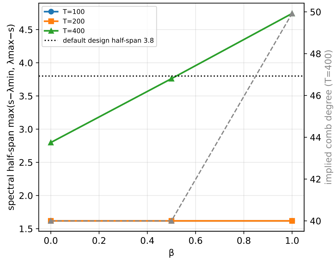
(c) the \beta cost: spectrum widens \rightarrow degree grows
