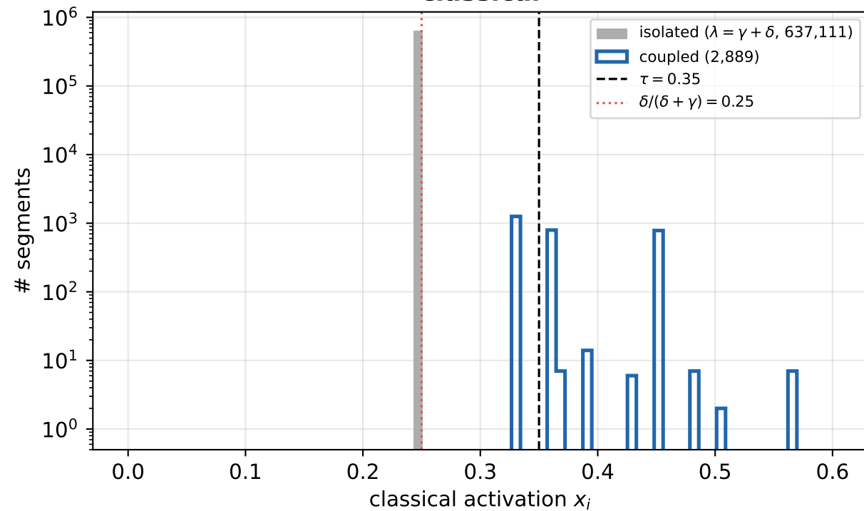
classical
