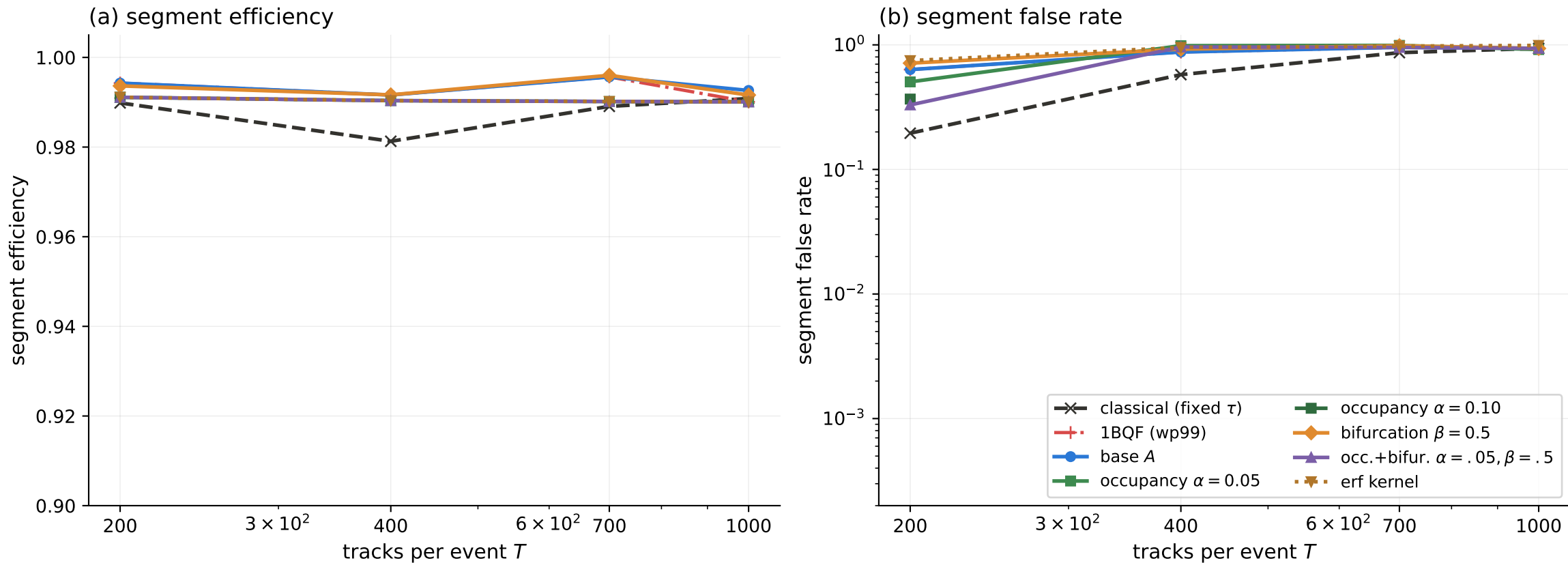
Segment metrics against track density — heavy noise (fitted response, d = 40 ; quantum at wp99, classical at fixed \tau )
