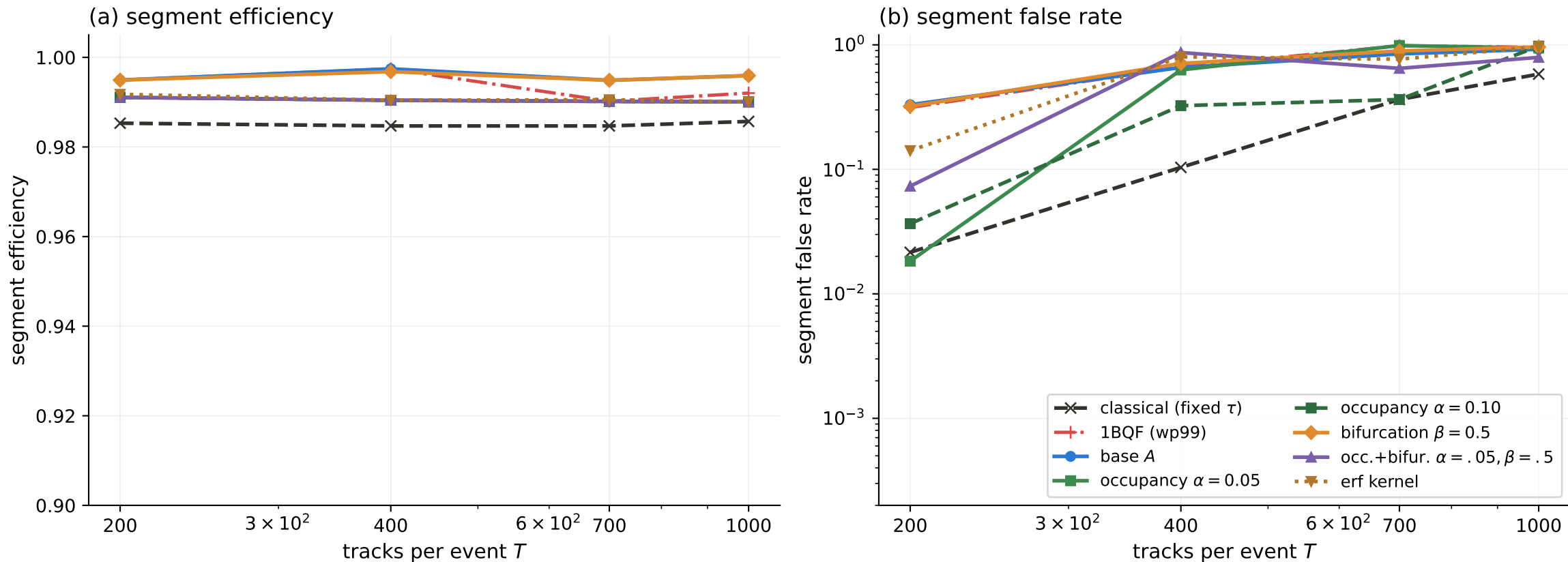
Segment metrics against track density — moderate noise (fitted response, d = 40 ; quantum at wp99, classical at fixed \tau )
